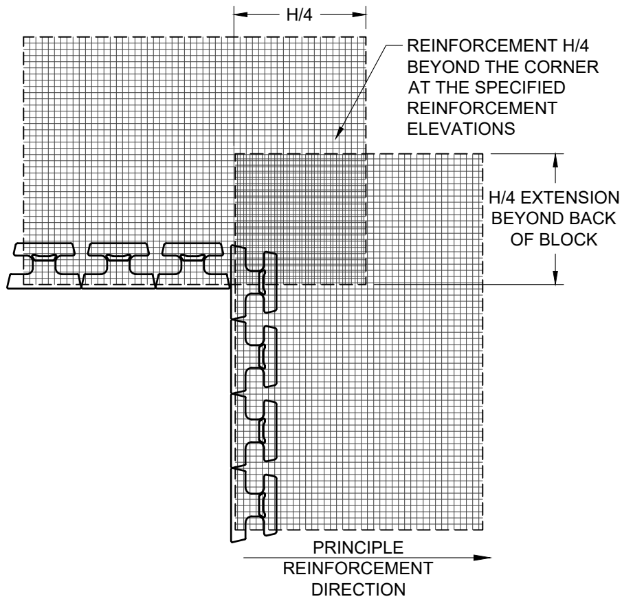
GEOGRID LAYOUT
