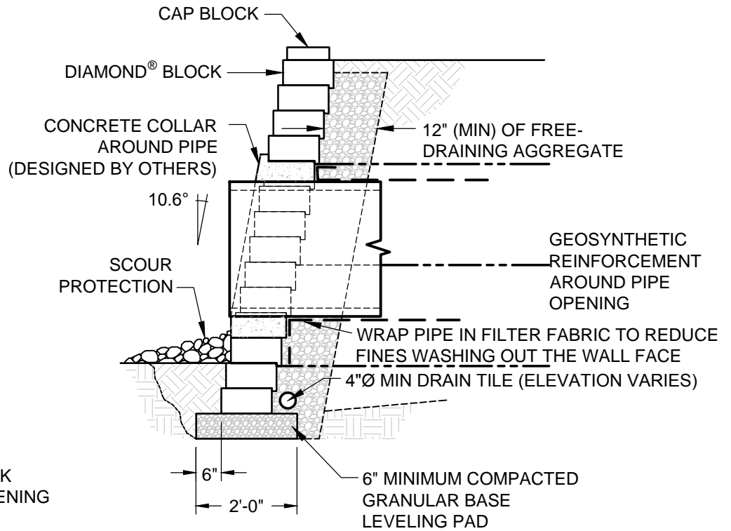
SECTION VIEW
