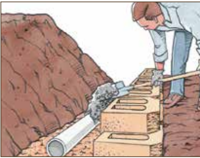
Diagram 4—Drainage
