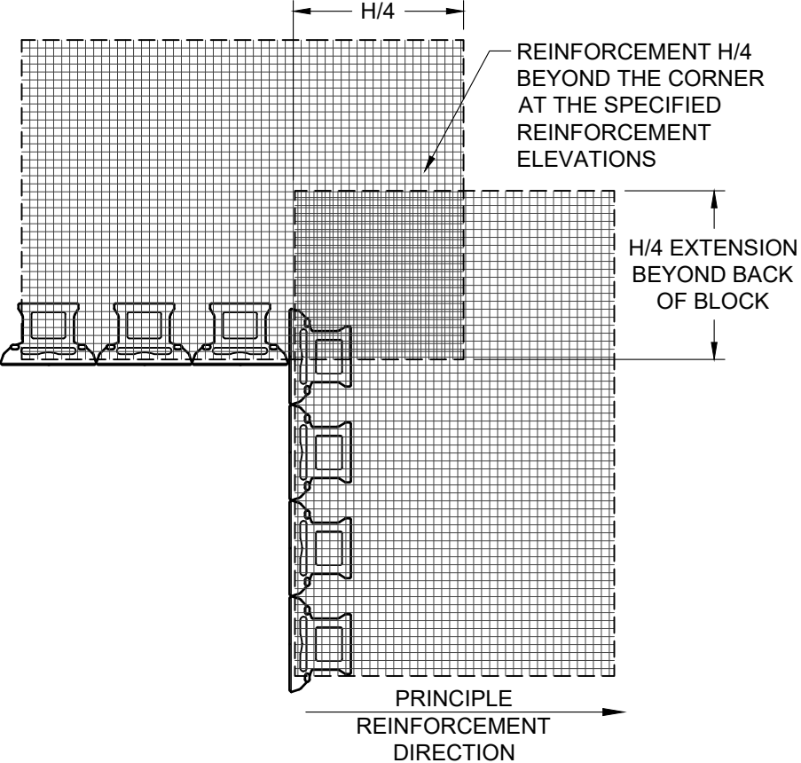
GEOGRID LAYOUT
