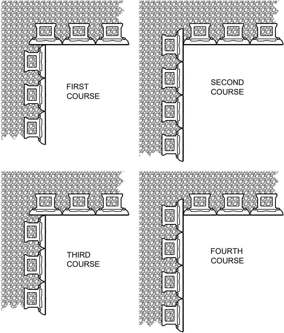
BLOCK LAYOUT
