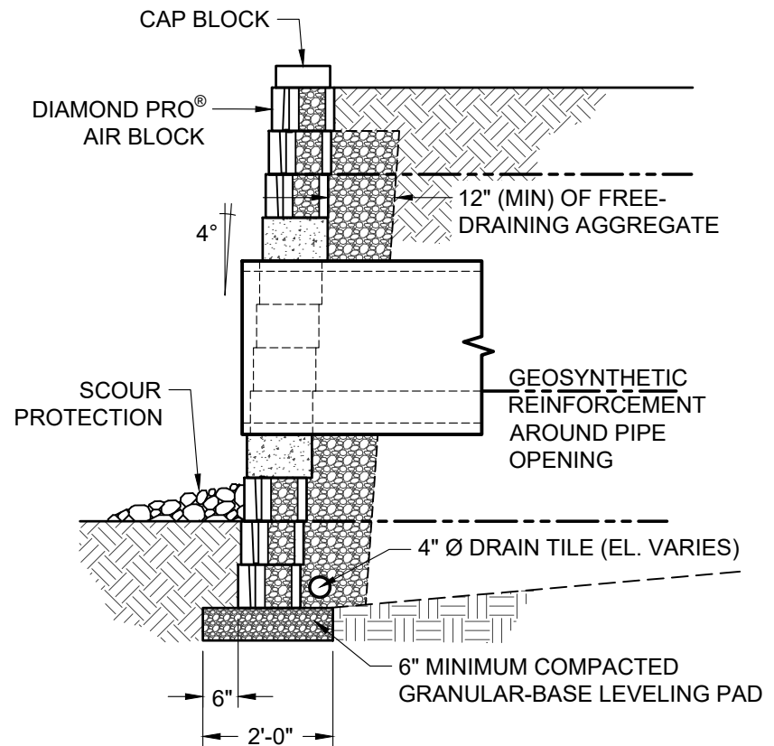
SECTION VIEW
