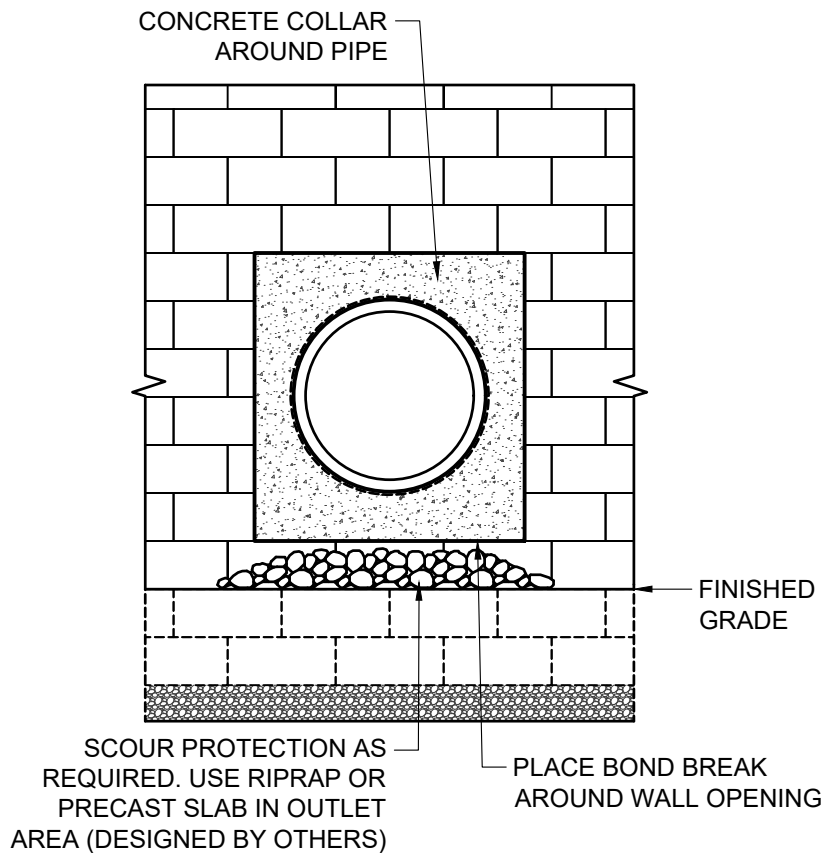
FACE VIEW
