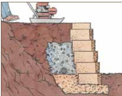
Diagram 6—Compaction
