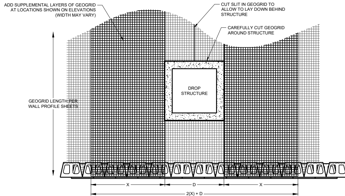
PLAN VIEW
