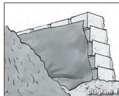
Filter fabric
