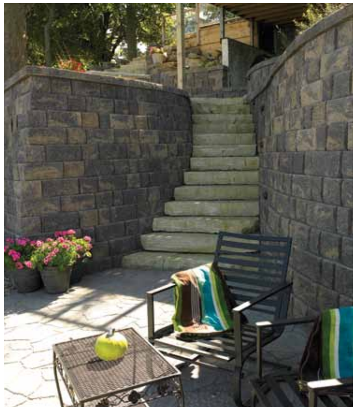
Terraced retaining walls transform a steep, dangerous slope on a small lot into a useful, safe and beautiful landscape.
